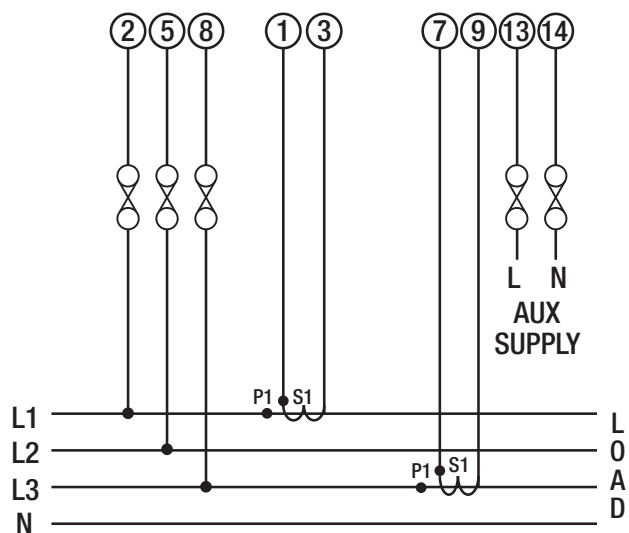
3-Phase 3-Wire unbalanced
